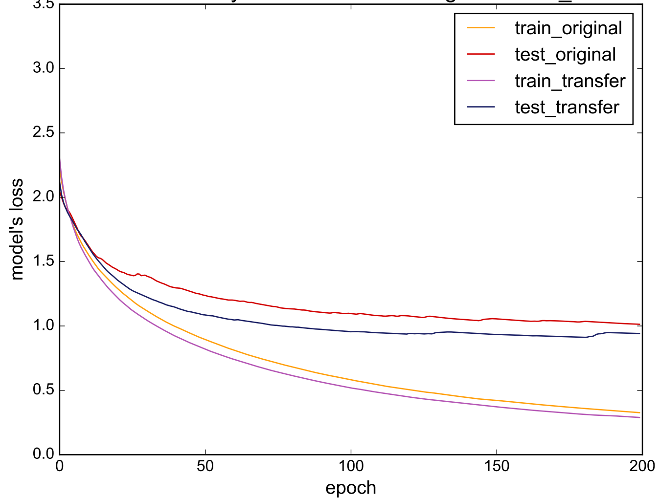
Source: ItalyPowerDemand - Target: Cricket_X
