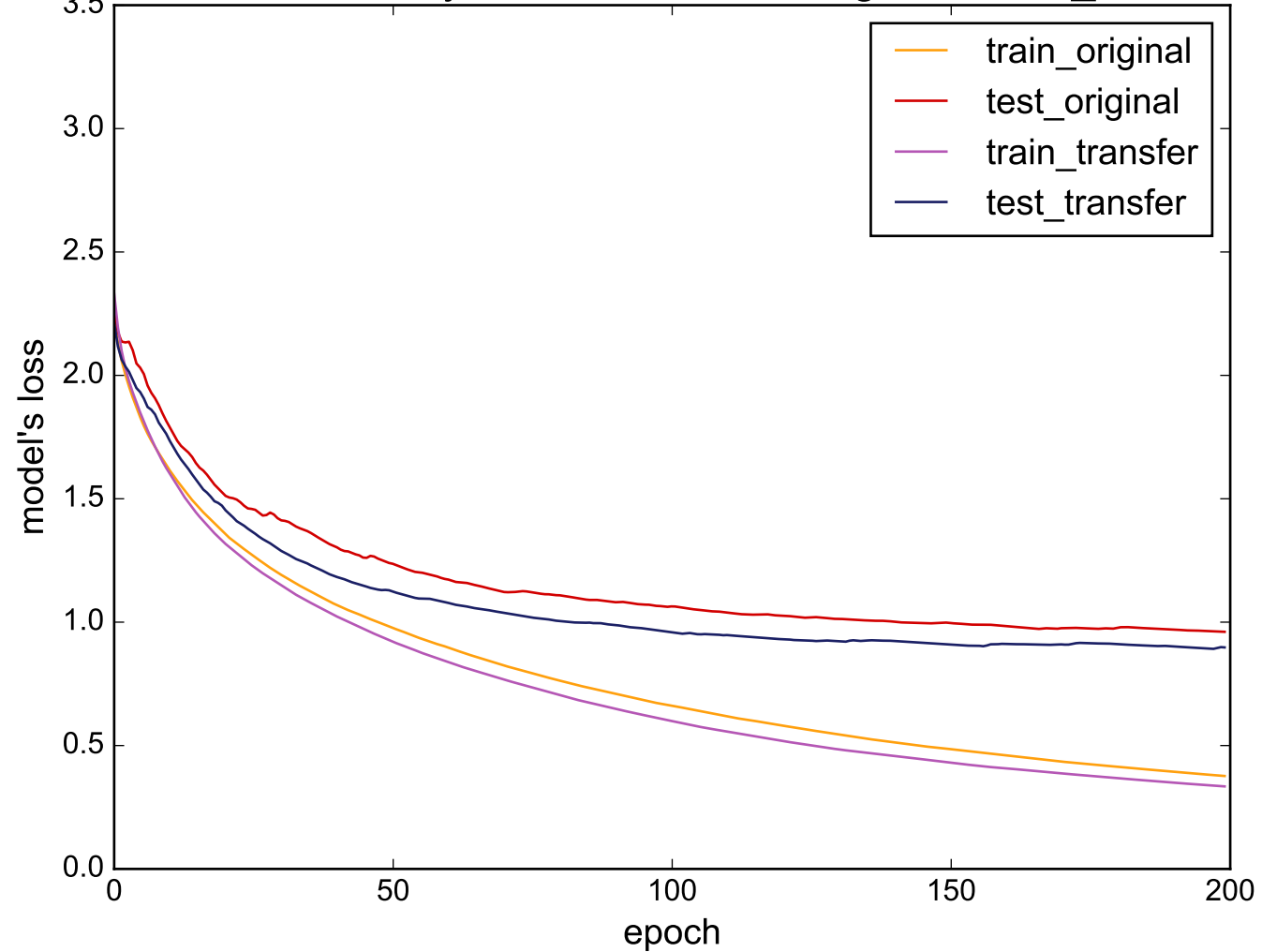
Source: ItalyPowerDemand - Target: Cricket_Z
