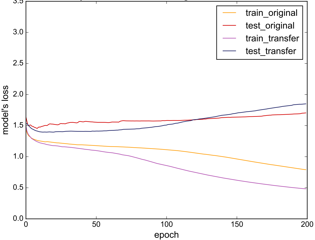
Source: ItalyPowerDemand - Target: DiatomSizeReduction
