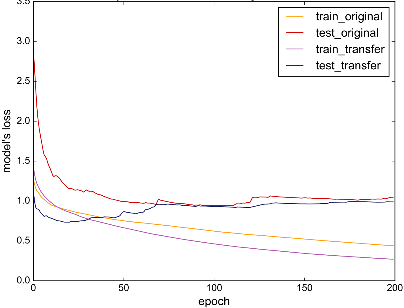
Source: ItalyPowerDemand - Target: DistalPhalanxTW
