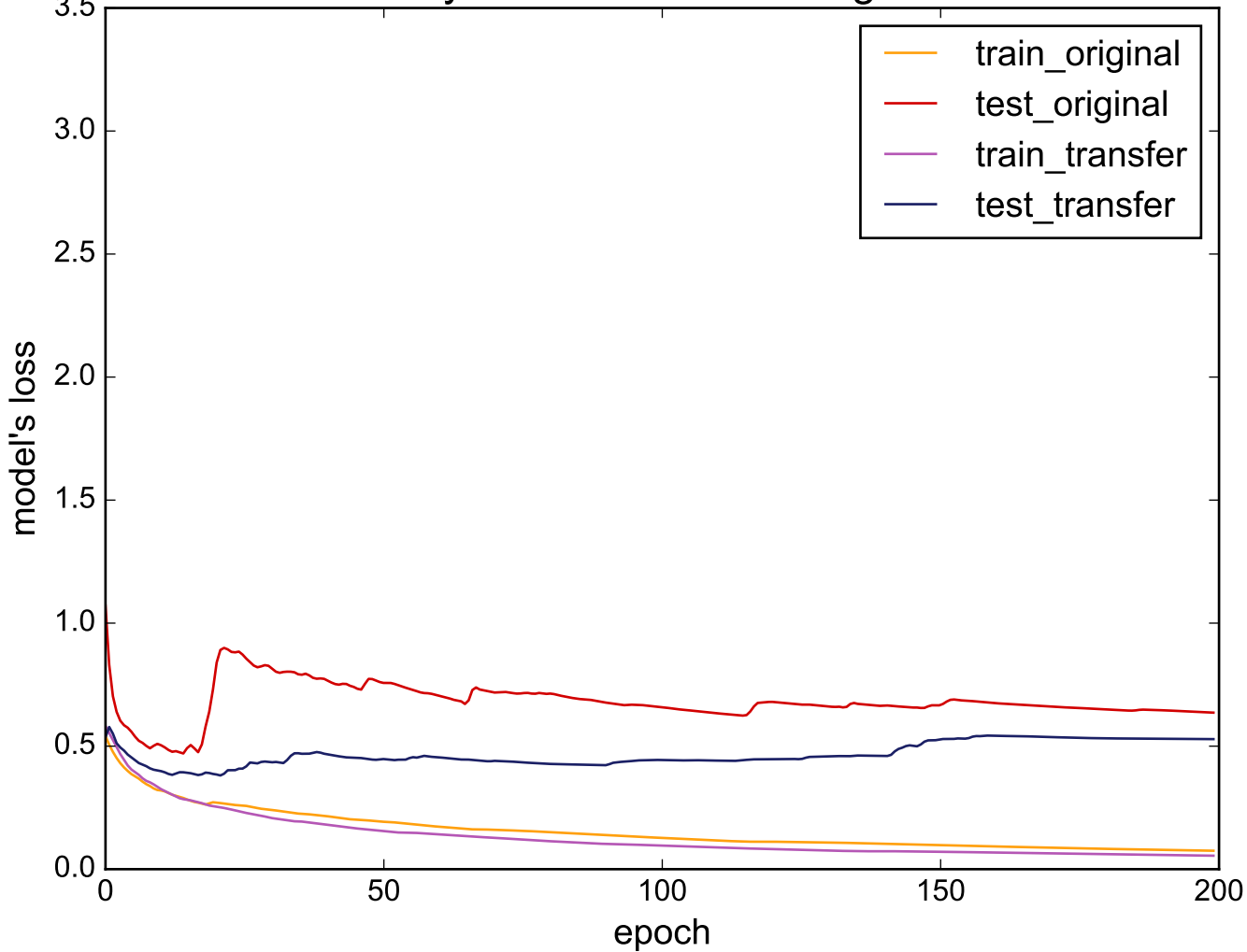
Source: ItalyPowerDemand - Target: ECG200
