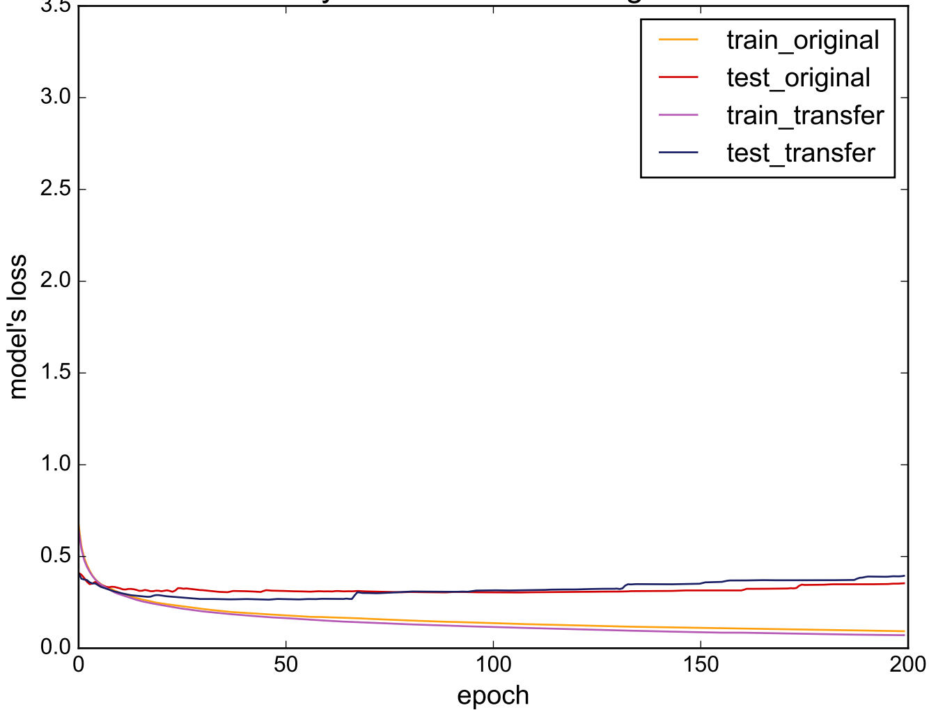
Source: ItalyPowerDemand - Target: ECG5000
