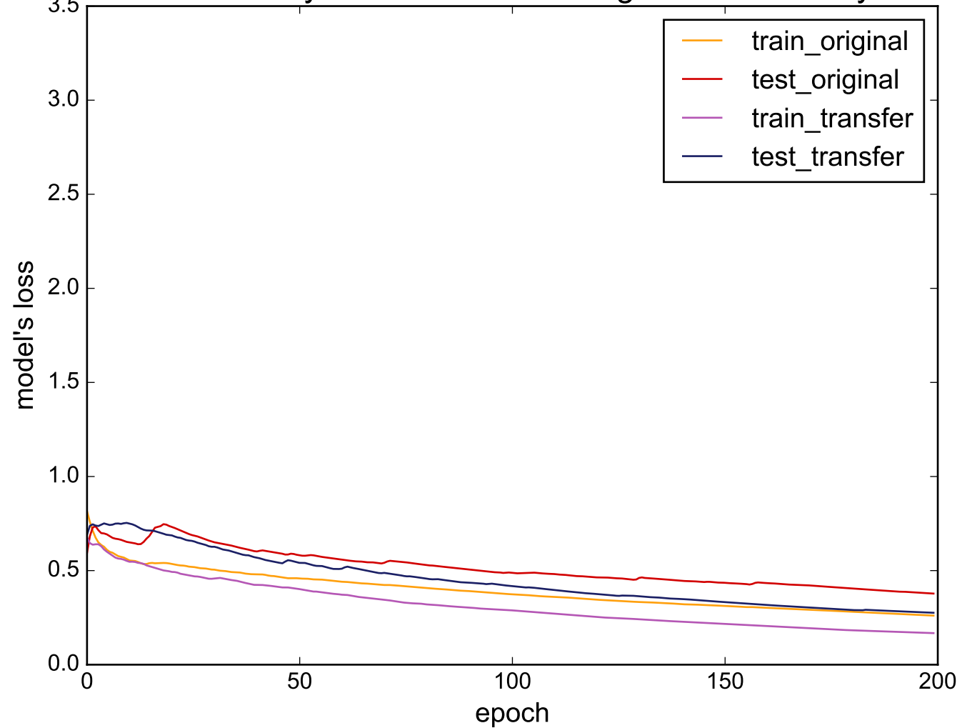
Source: ItalyPowerDemand - Target: ECGFiveDays
