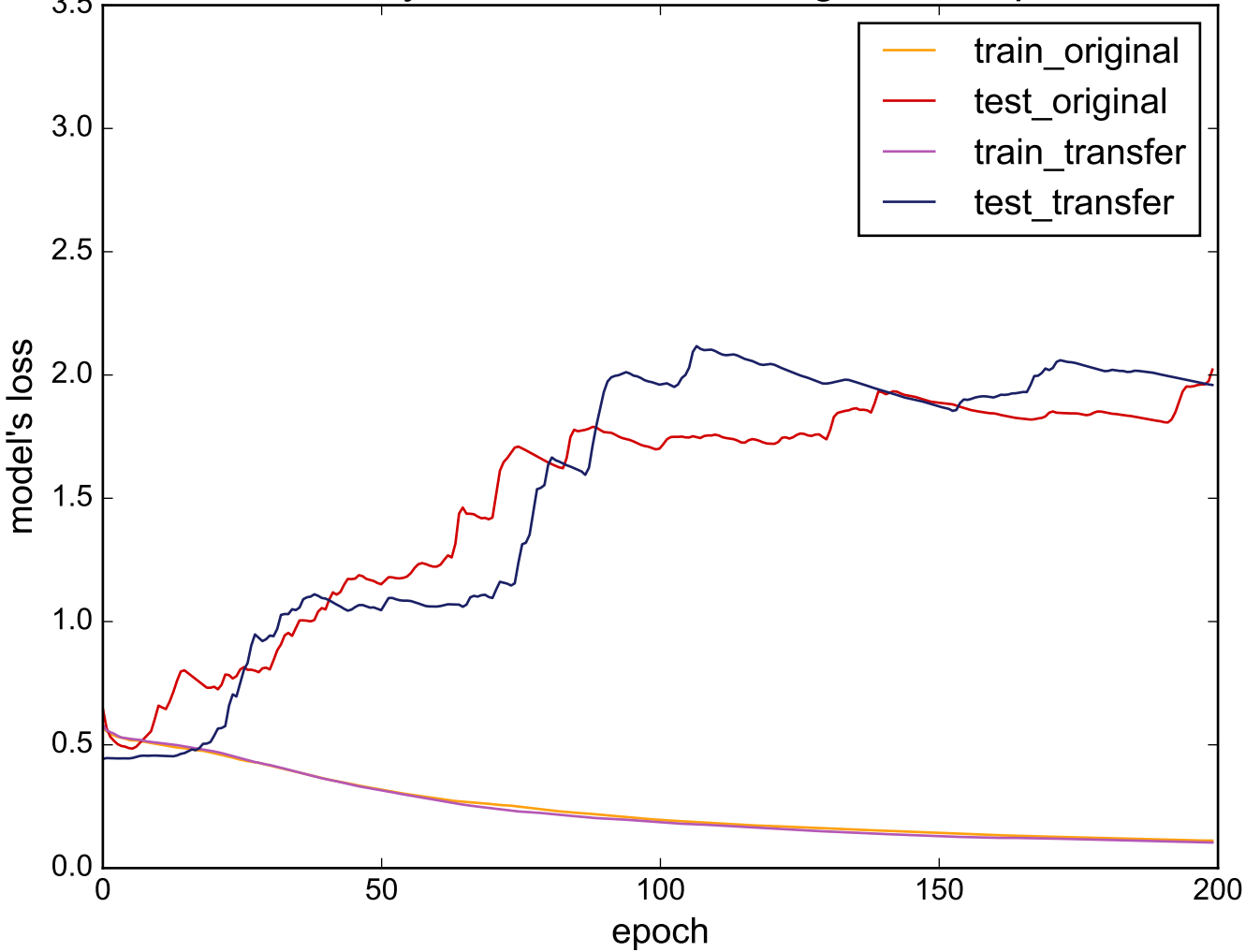
Source: ItalyPowerDemand - Target: Earthquakes
