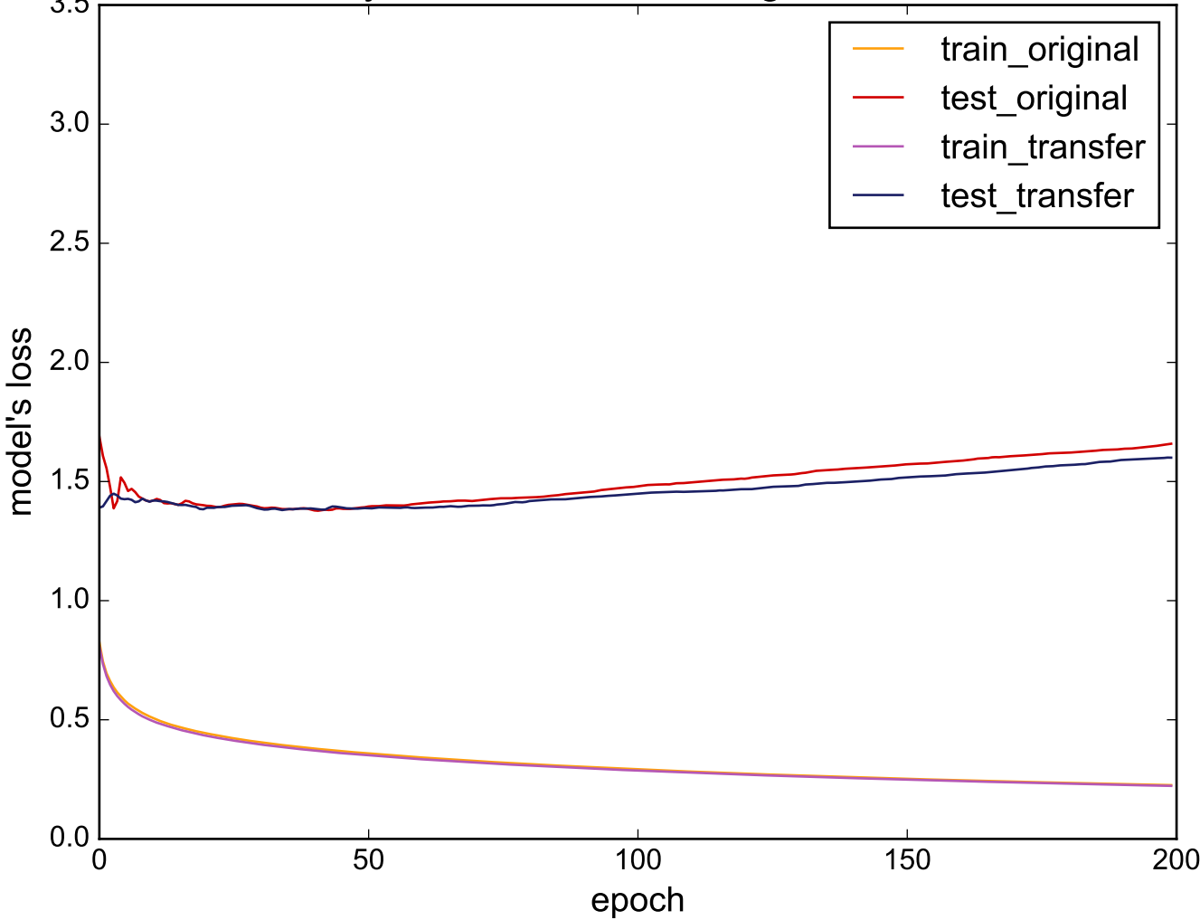
Source: ItalyPowerDemand - Target: ElectricDevices
