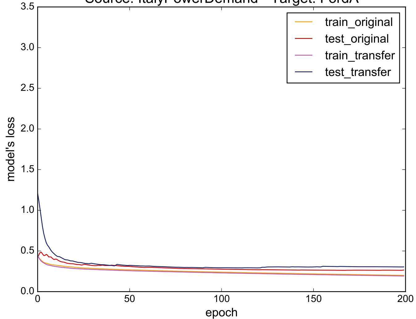
Source: ItalyPowerDemand - Target: FordA
