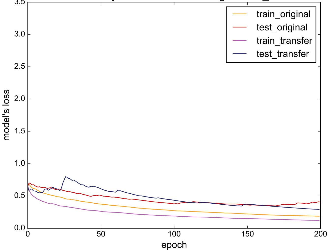
Source: ItalyPowerDemand - Target: Gun_Point
