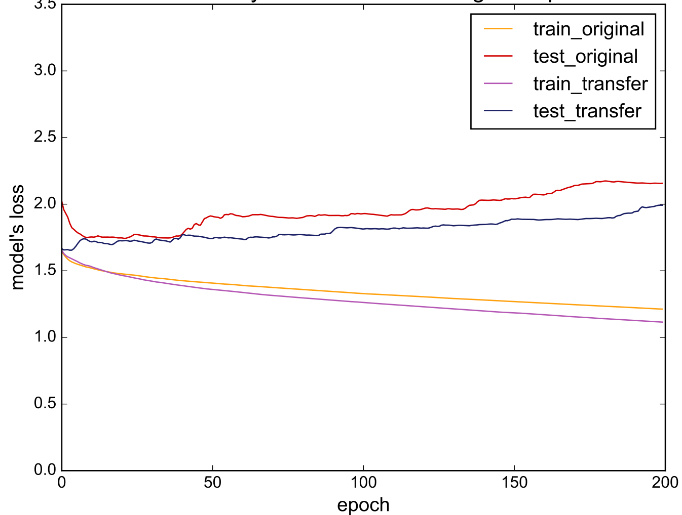
Source: ItalyPowerDemand - Target: Haptics
