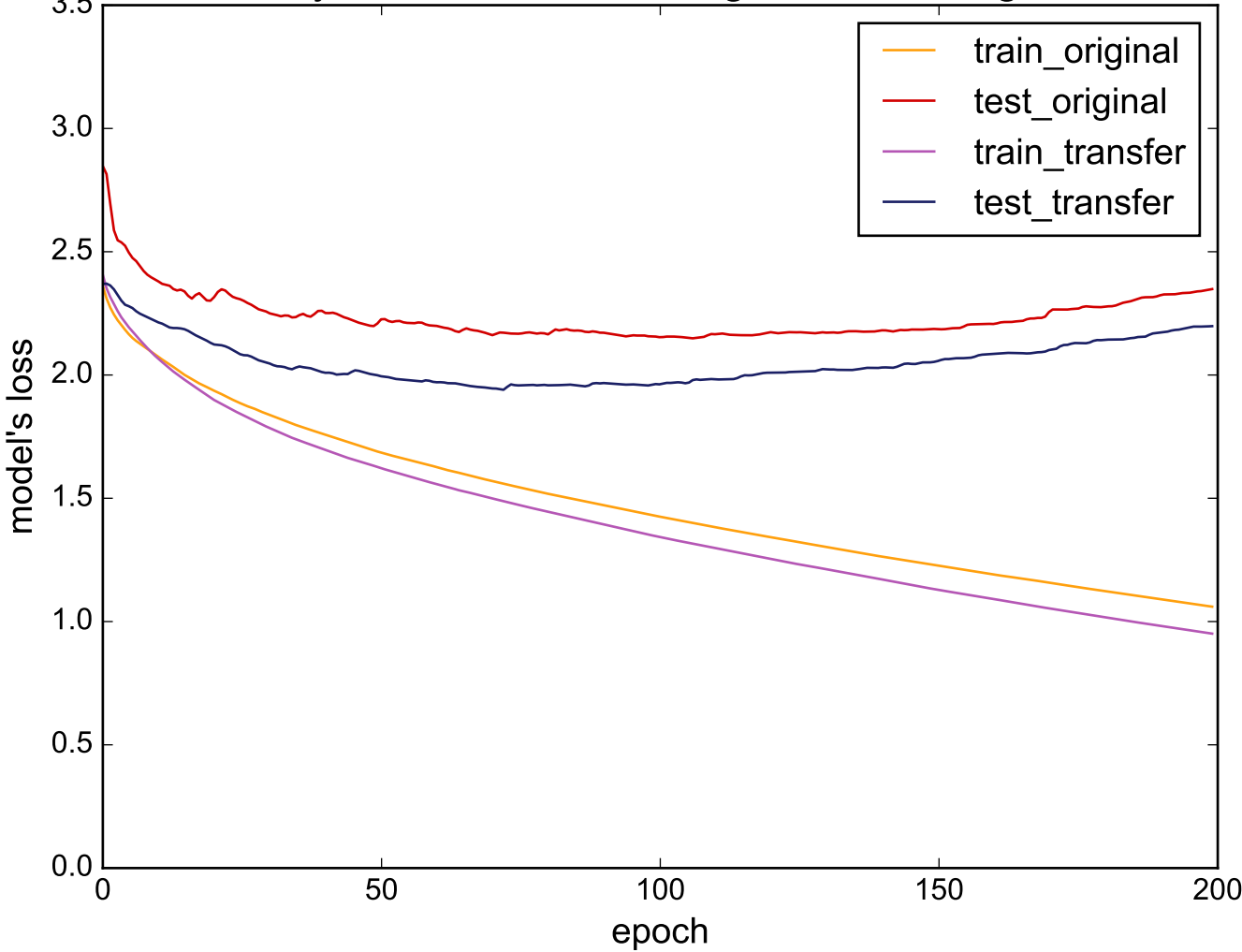
Source: ItalyPowerDemand - Target: InsectWingbeatSound
