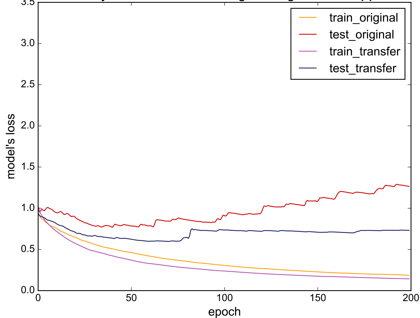
Source: ItalyPowerDemand - Target: LargeKitchenAppliances
