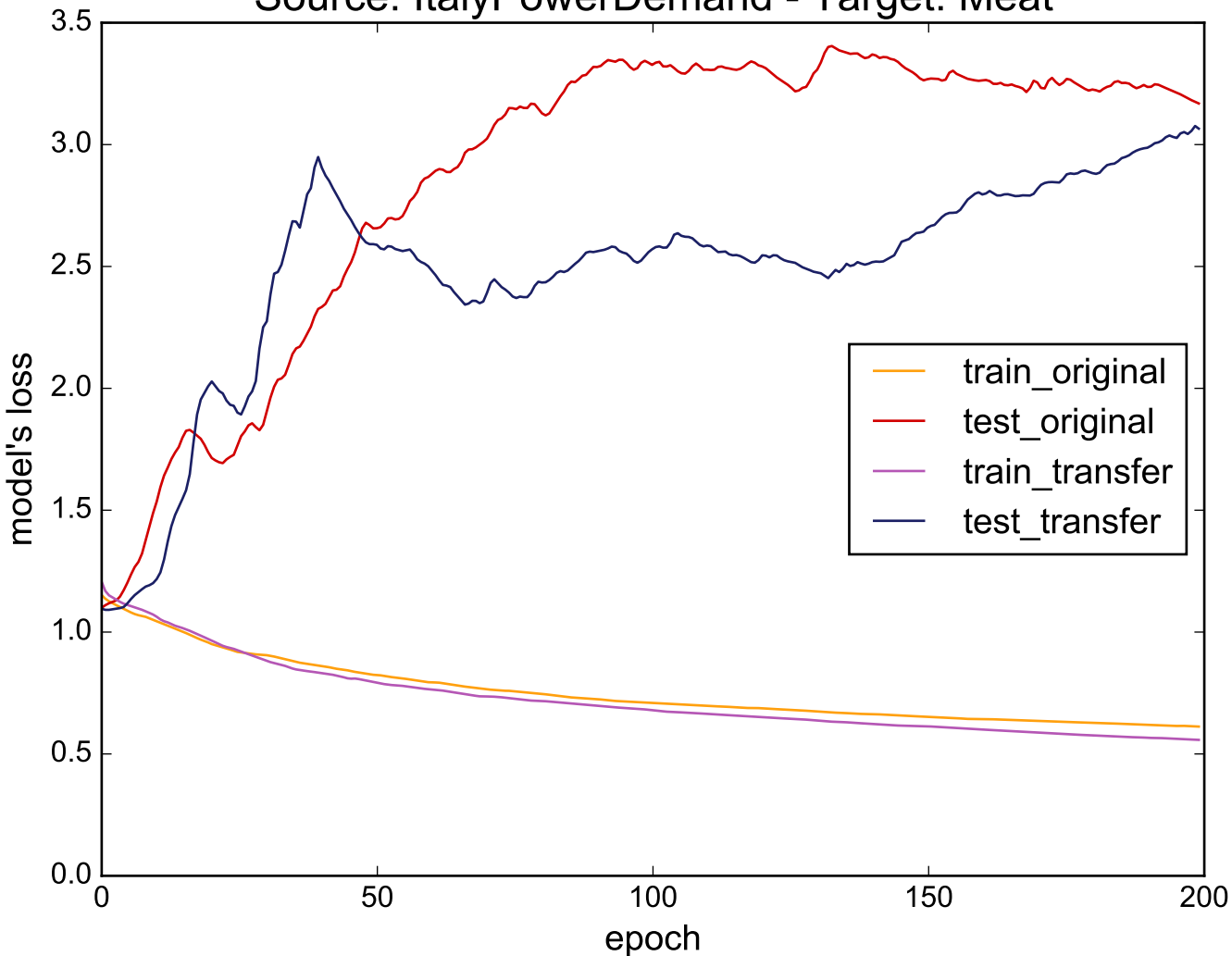
Source: ItalyPowerDemand - Target: Meat
