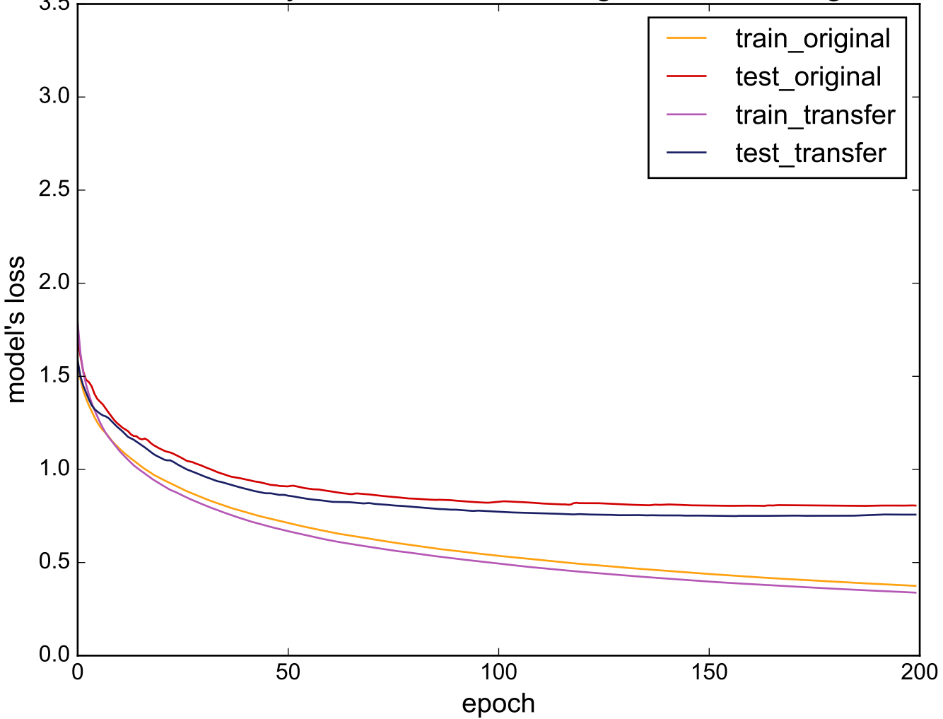
Source: ItalyPowerDemand - Target: MedicalImages
