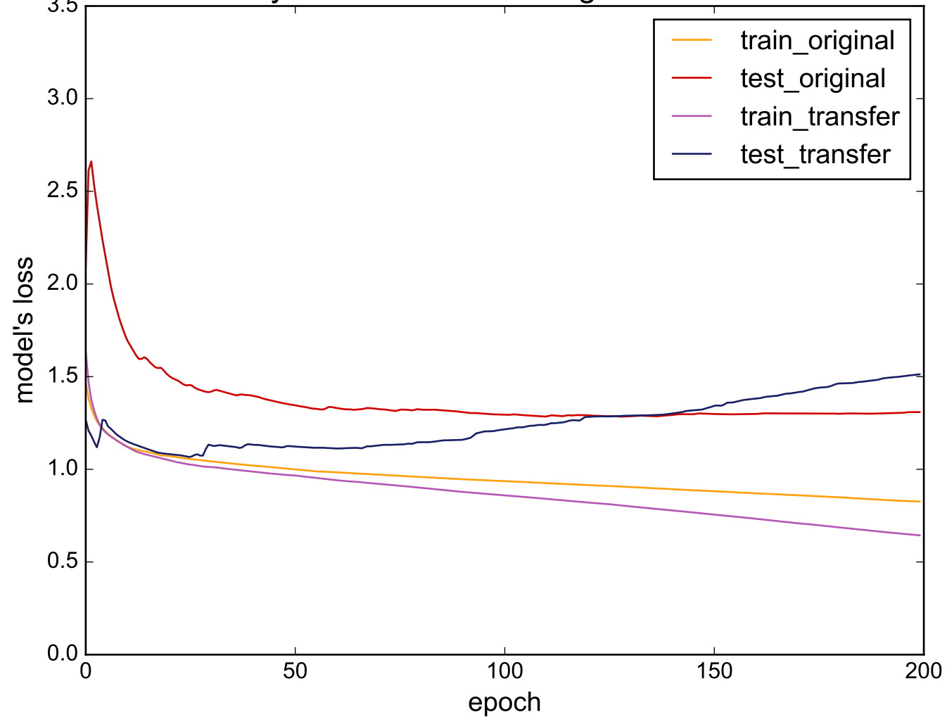
Source: ItalyPowerDemand - Target: MiddlePhalanxTW
