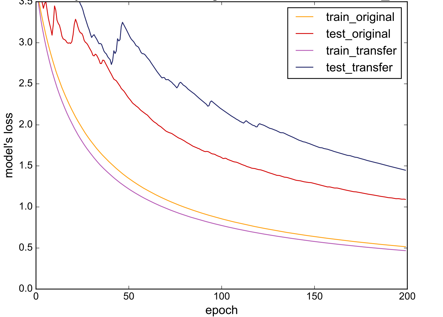
Source: ItalyPowerDemand - Target: NonInvasiveFetalECG_Thorax1
