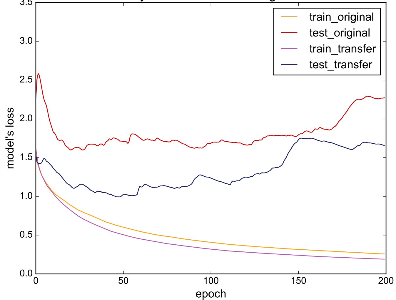
Source: ItalyPowerDemand - Target: OSULeaf
