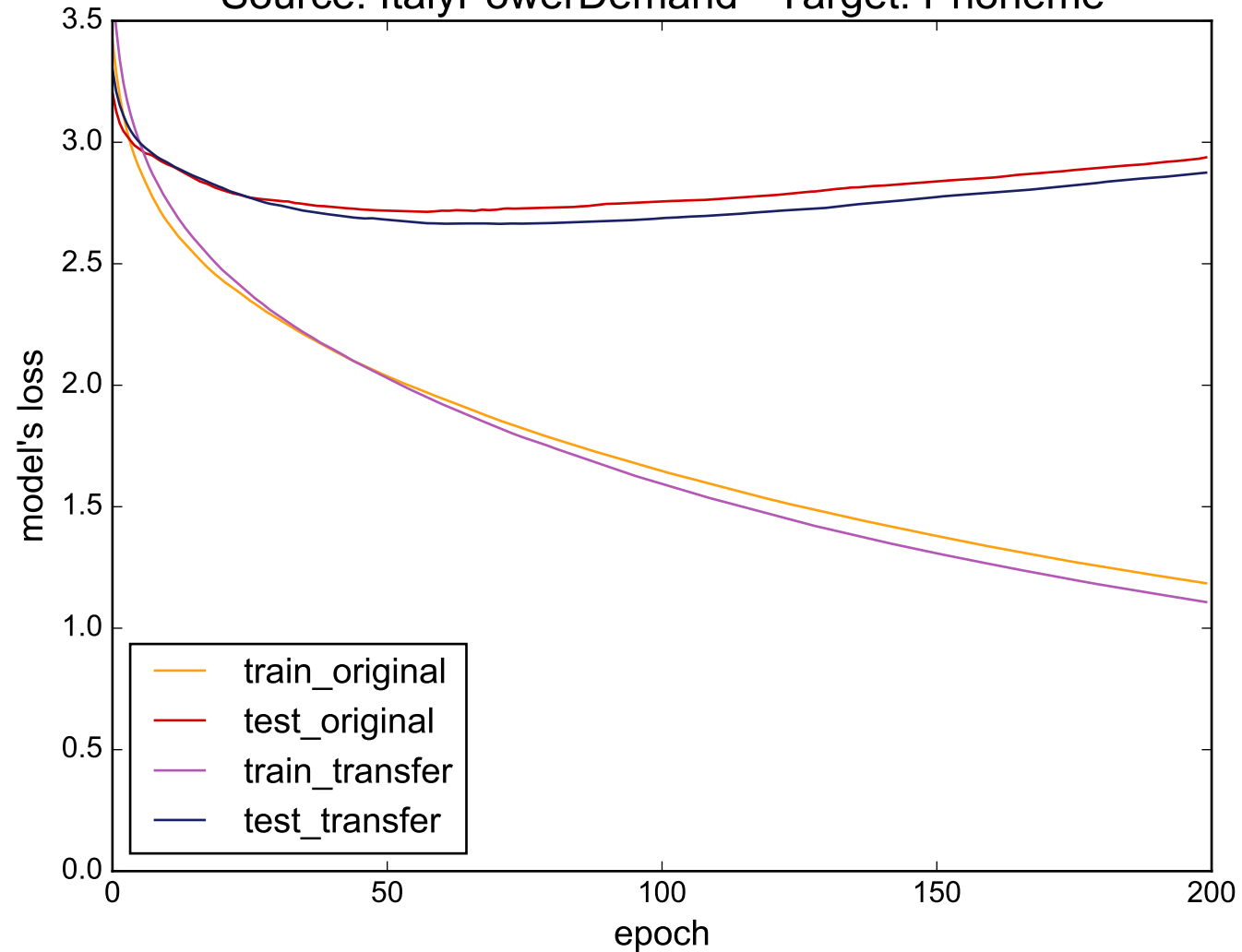
Source: ItalyPowerDemand - Target: Phoneme
