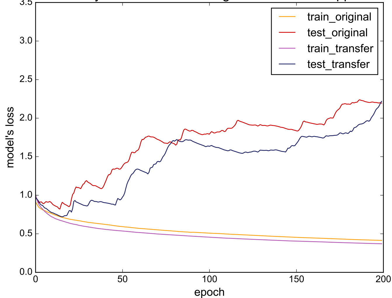
Source: ItalyPowerDemand - Target: SmallKitchenAppliances
