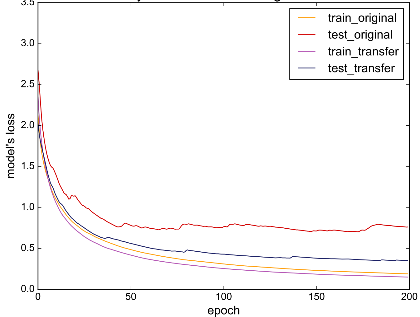
Source: ItalyPowerDemand - Target: SwedishLeaf
