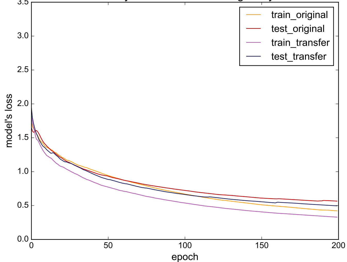
Source: ItalyPowerDemand - Target: Symbols
