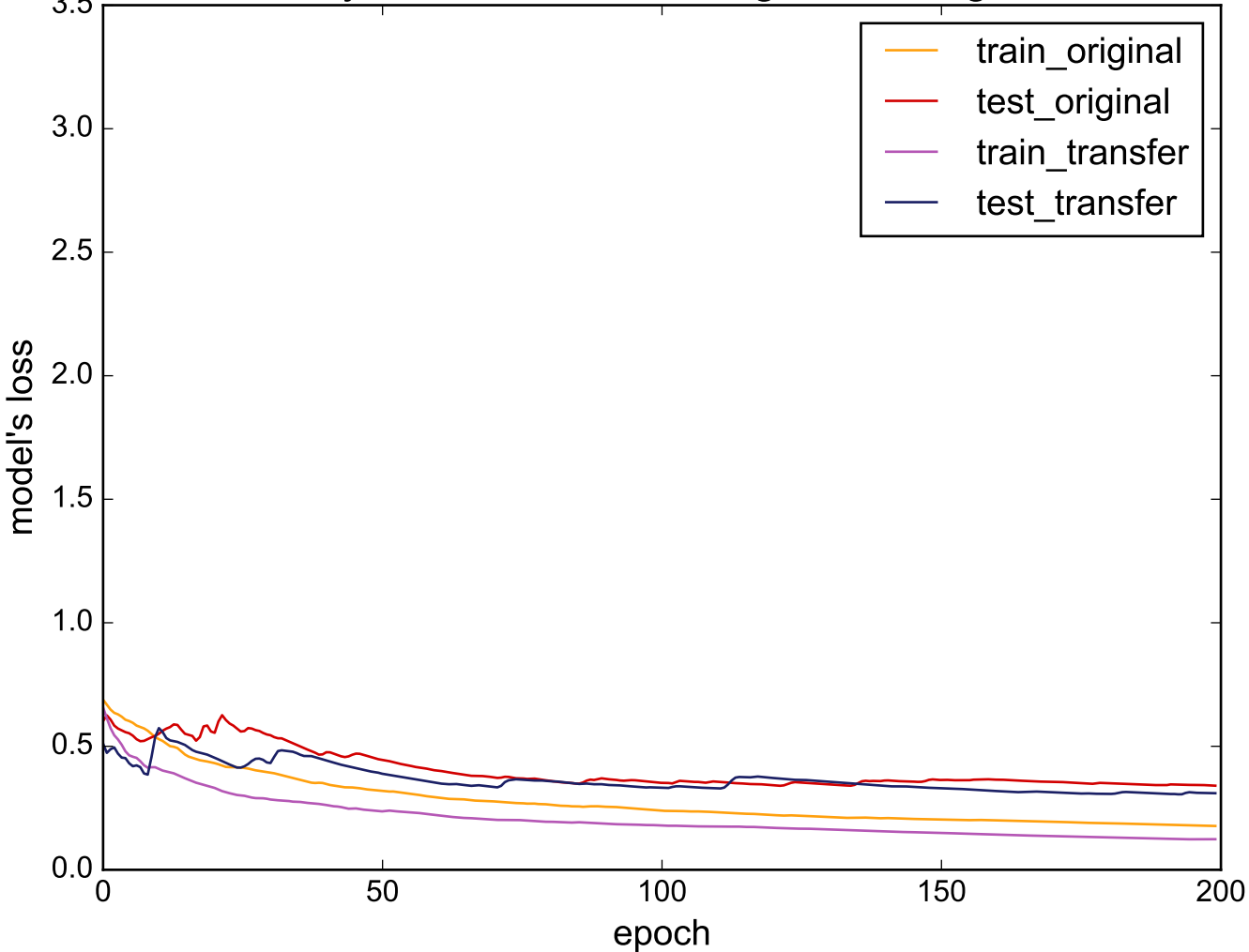
Source: ItalyPowerDemand - Target: ToeSegmentation1
