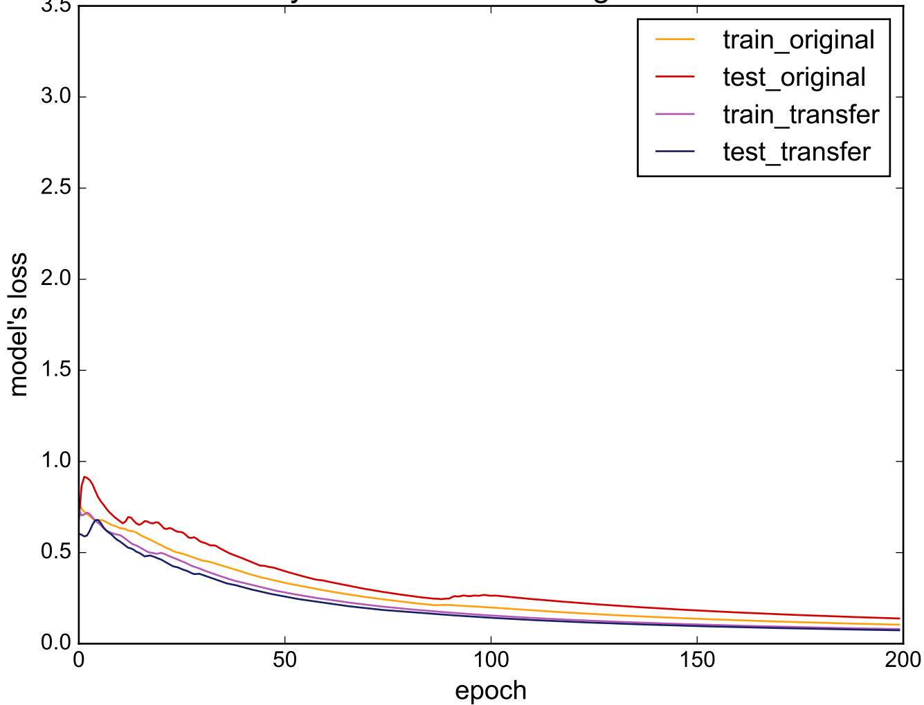
Source: ItalyPowerDemand - Target: TwoLeadECG
