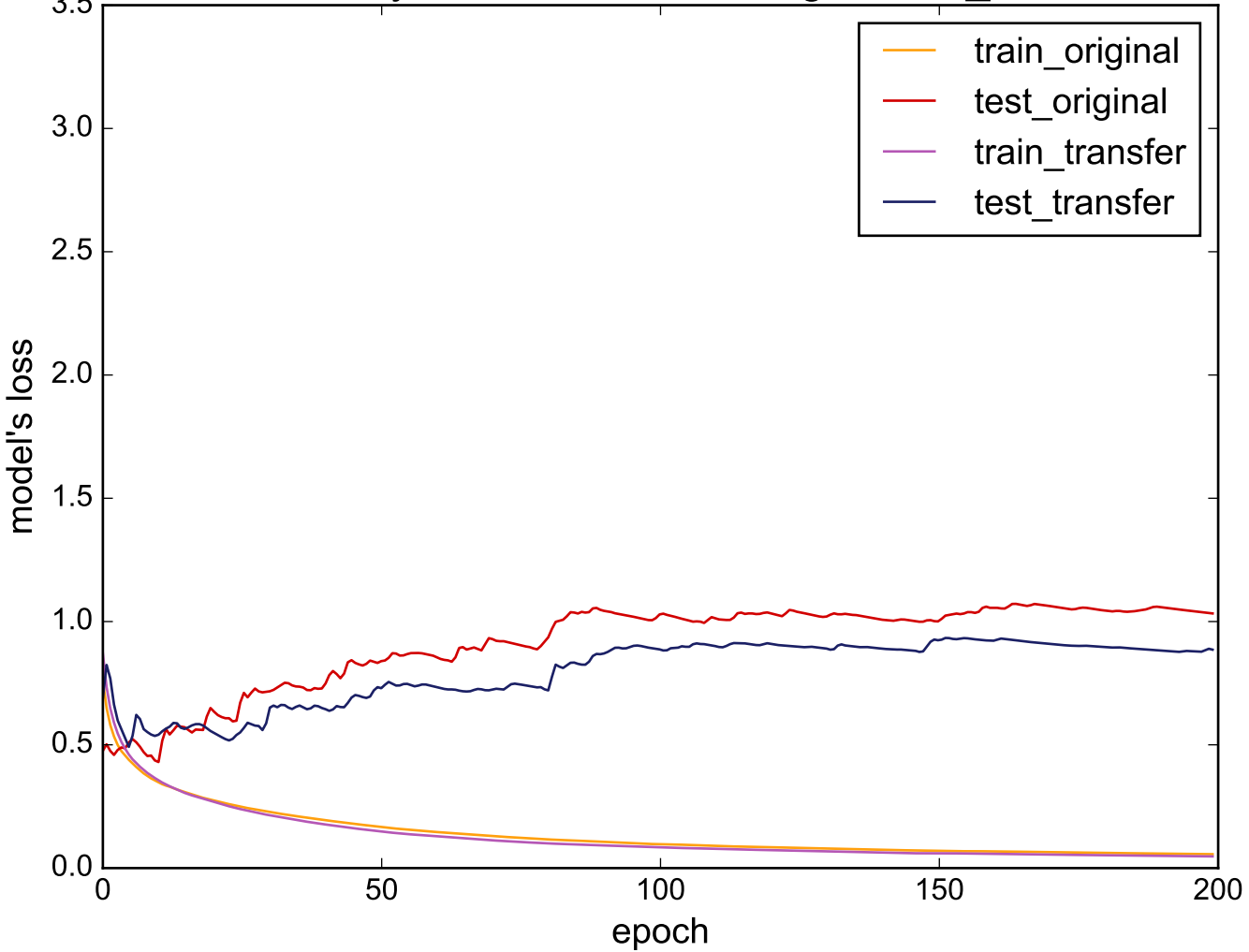
Source: ItalyPowerDemand - Target: Two_Patterns
