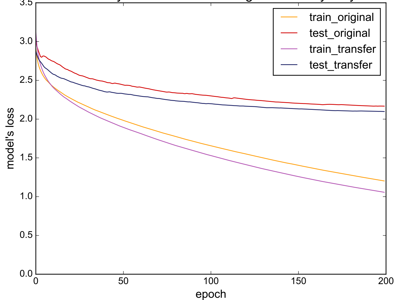
Source: ItalyPowerDemand - Target: WordsSynonyms
