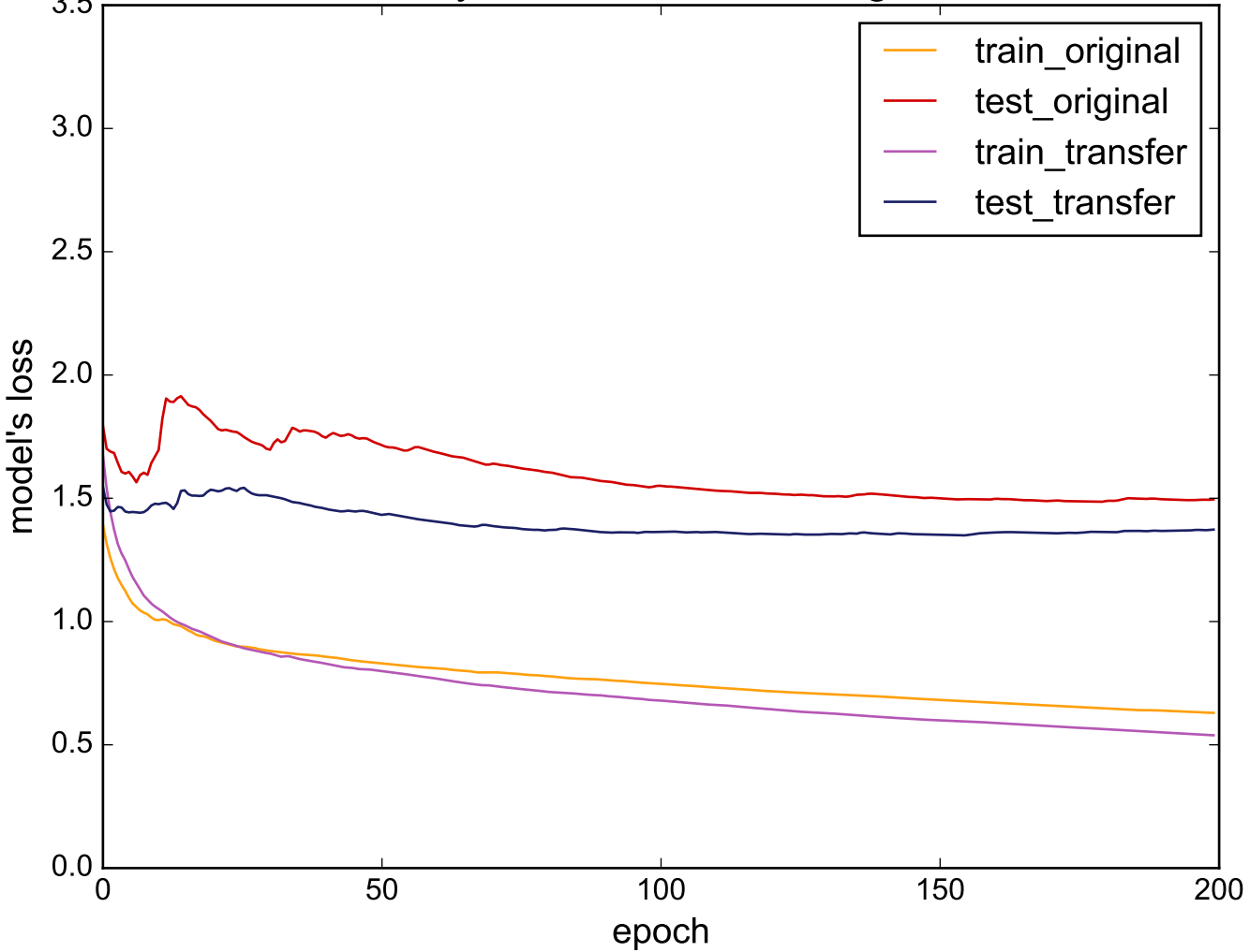
Source: ItalyPowerDemand - Target: Worms
