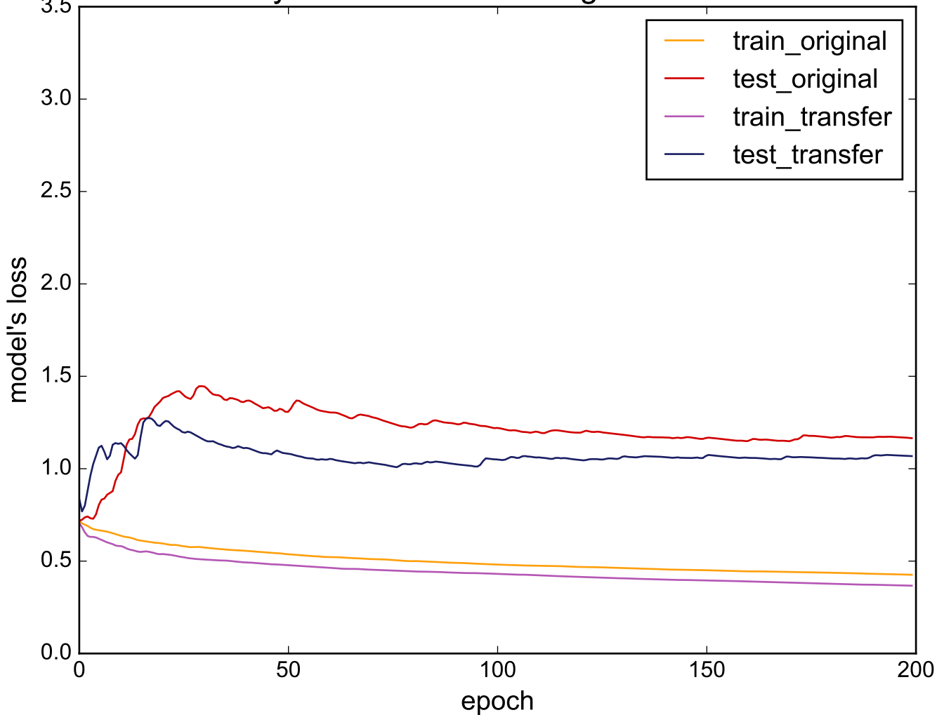
Source: ItalyPowerDemand - Target: WormsTwoClass
