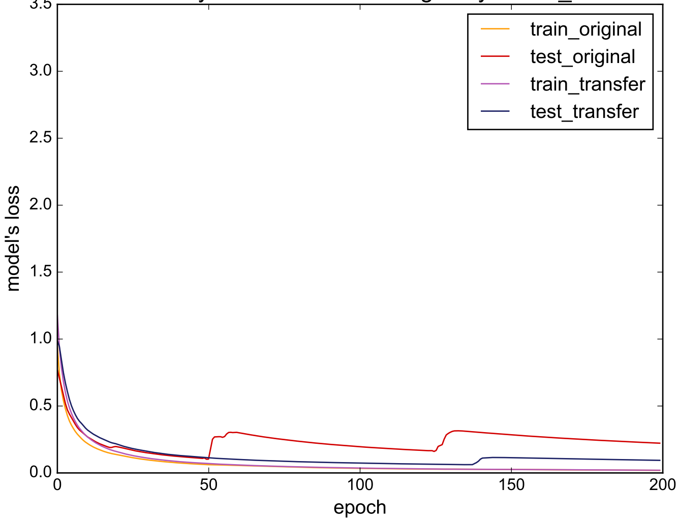
Source: ItalyPowerDemand - Target: synthetic_control
