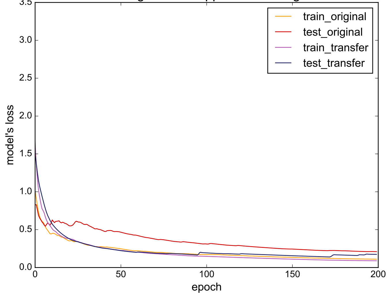
Source: LargeKitchenAppliances - Target: CBF
