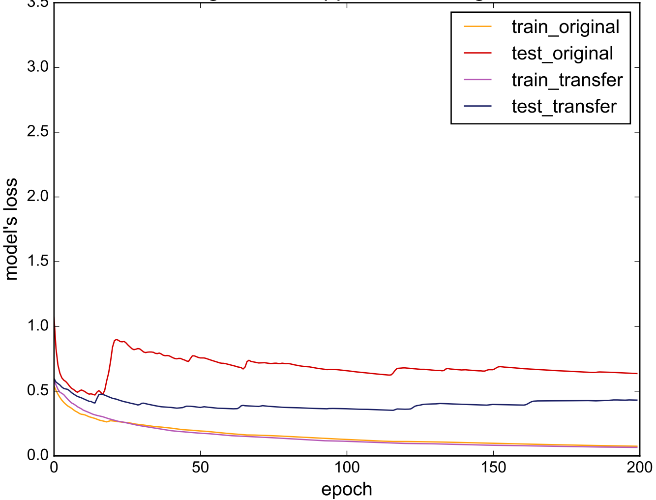
Source: LargeKitchenAppliances - Target: ECG200
