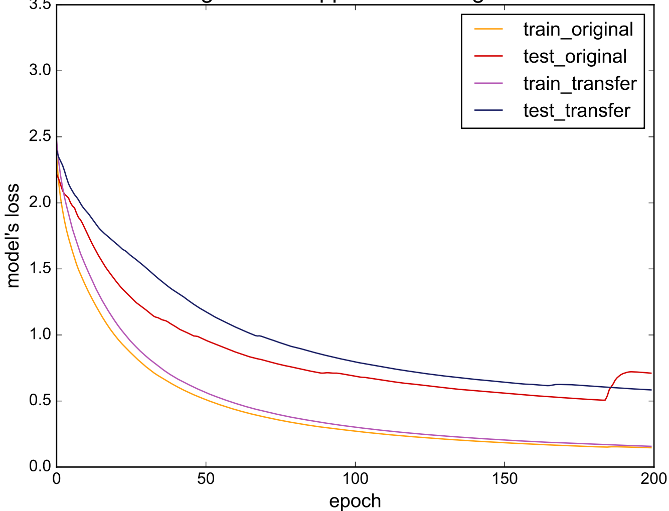
Source: LargeKitchenAppliances - Target: FacesUCR
