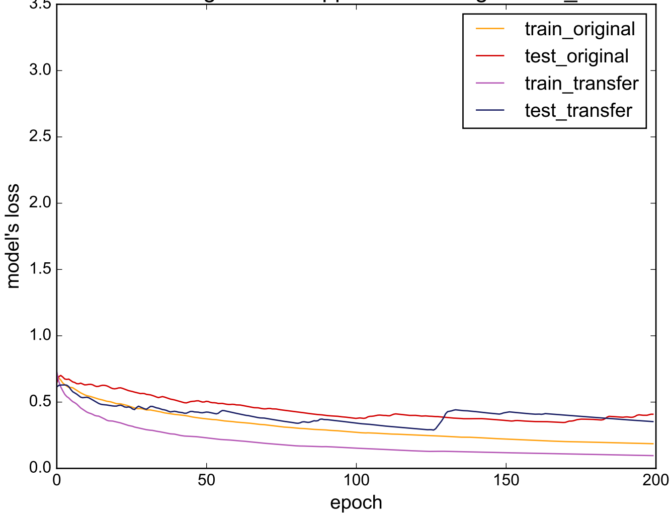
Source: LargeKitchenAppliances - Target: Gun_Point
