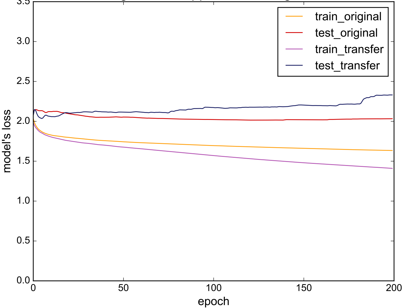
Source: LargeKitchenAppliances - Target: InlineSkate
