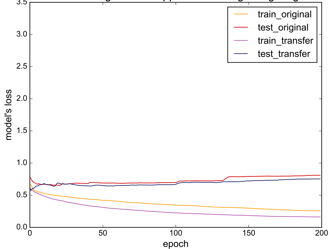
Source: LargeKitchenAppliances - Target: Lighting2
