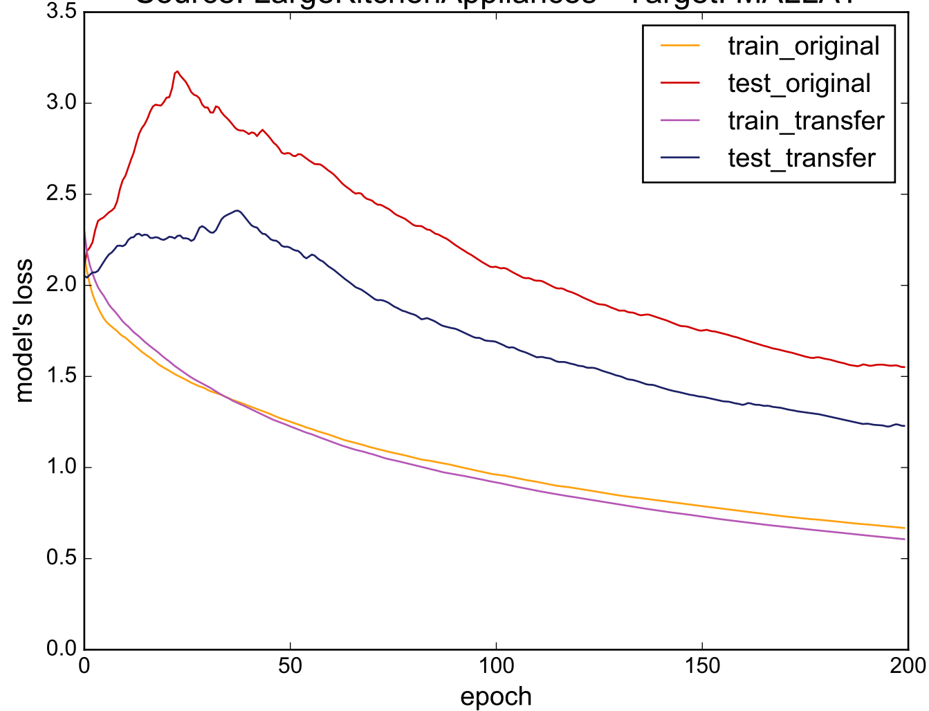
Source: LargeKitchenAppliances - Target: MALLAT
