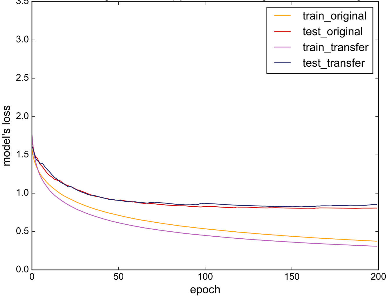
Source: LargeKitchenAppliances - Target: MedicalImages
