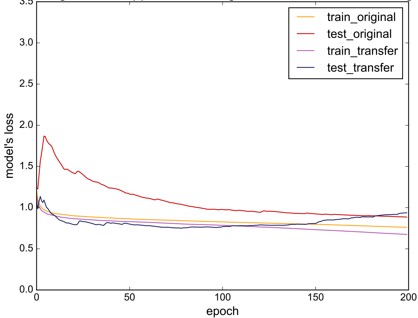
Source: LargeKitchenAppliances - Target: MiddlePhalanxOutlineAgeGroup
