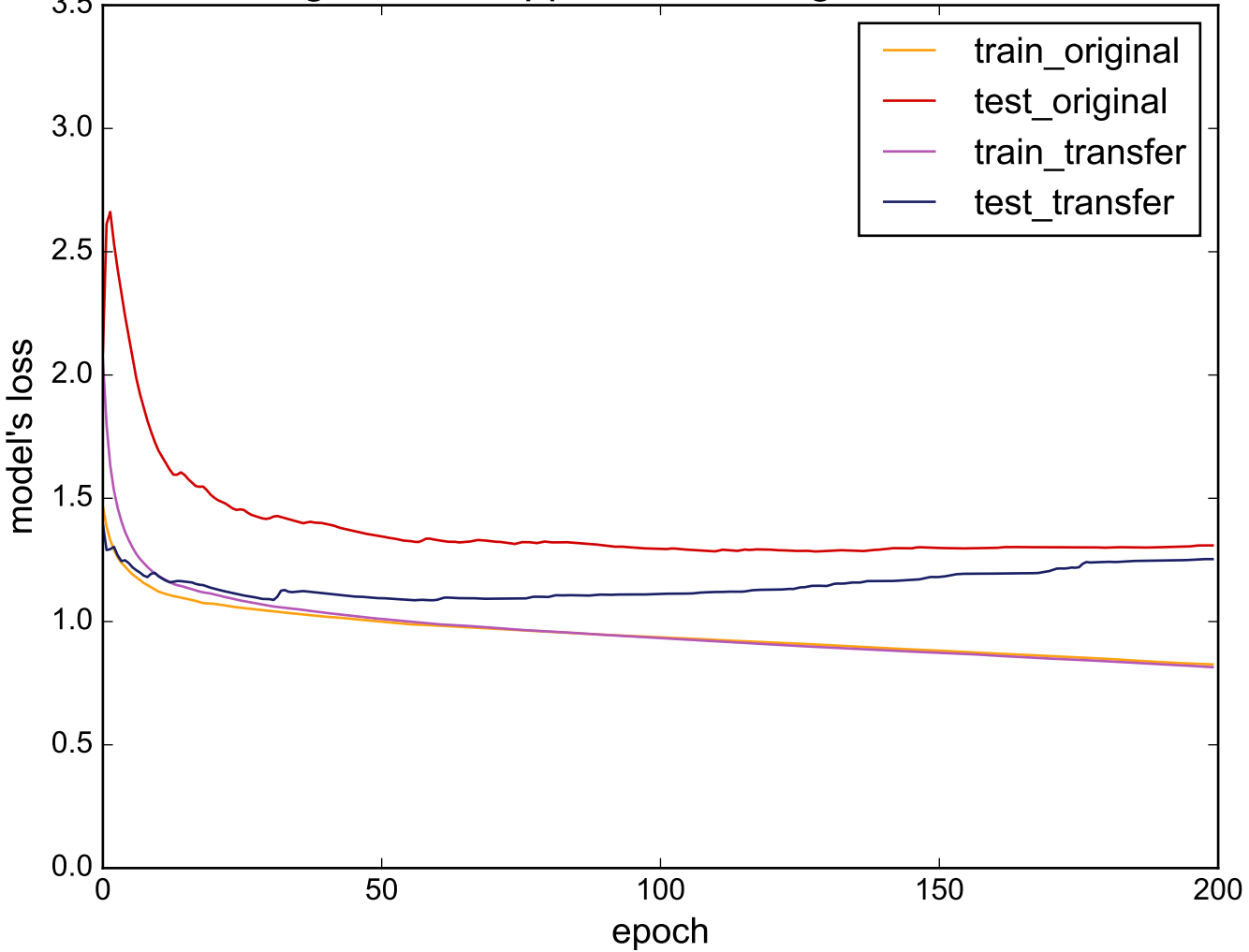
Source: LargeKitchenAppliances - Target: MiddlePhalanxTW
