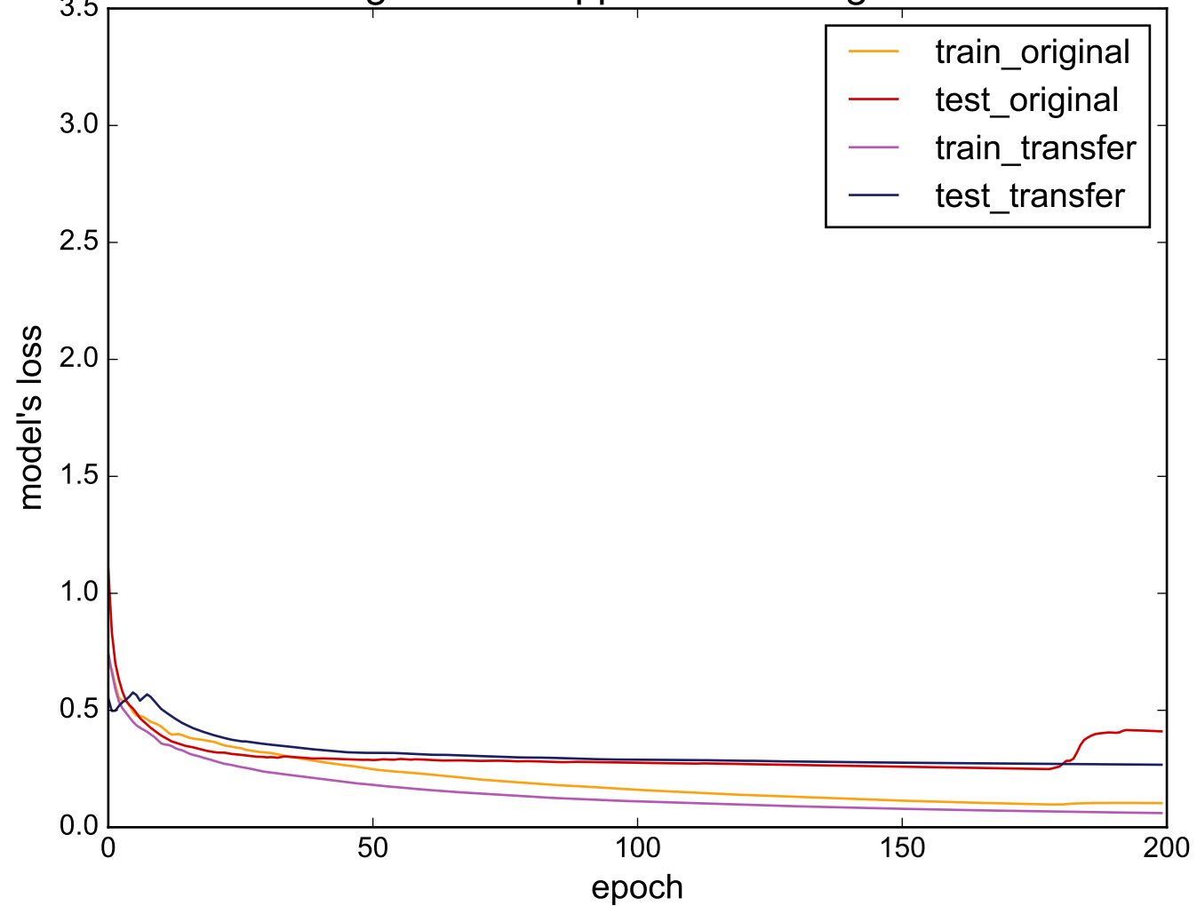
Source: LargeKitchenAppliances - Target: MoteStrain
