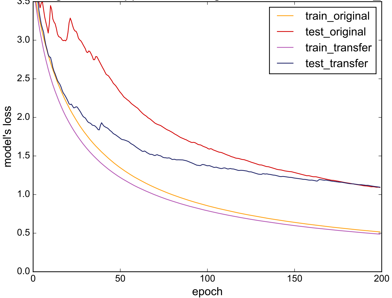
Source: LargeKitchenAppliances - Target: NonInvasiveFetalECG_Thorax1
