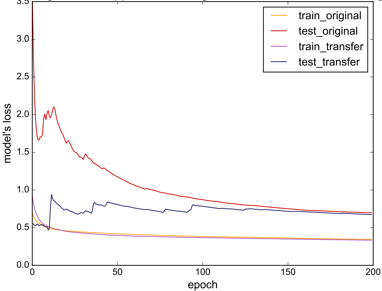
Source: LargeKitchenAppliances - Target: ProximalPhalanxOutlineAgeGroup
