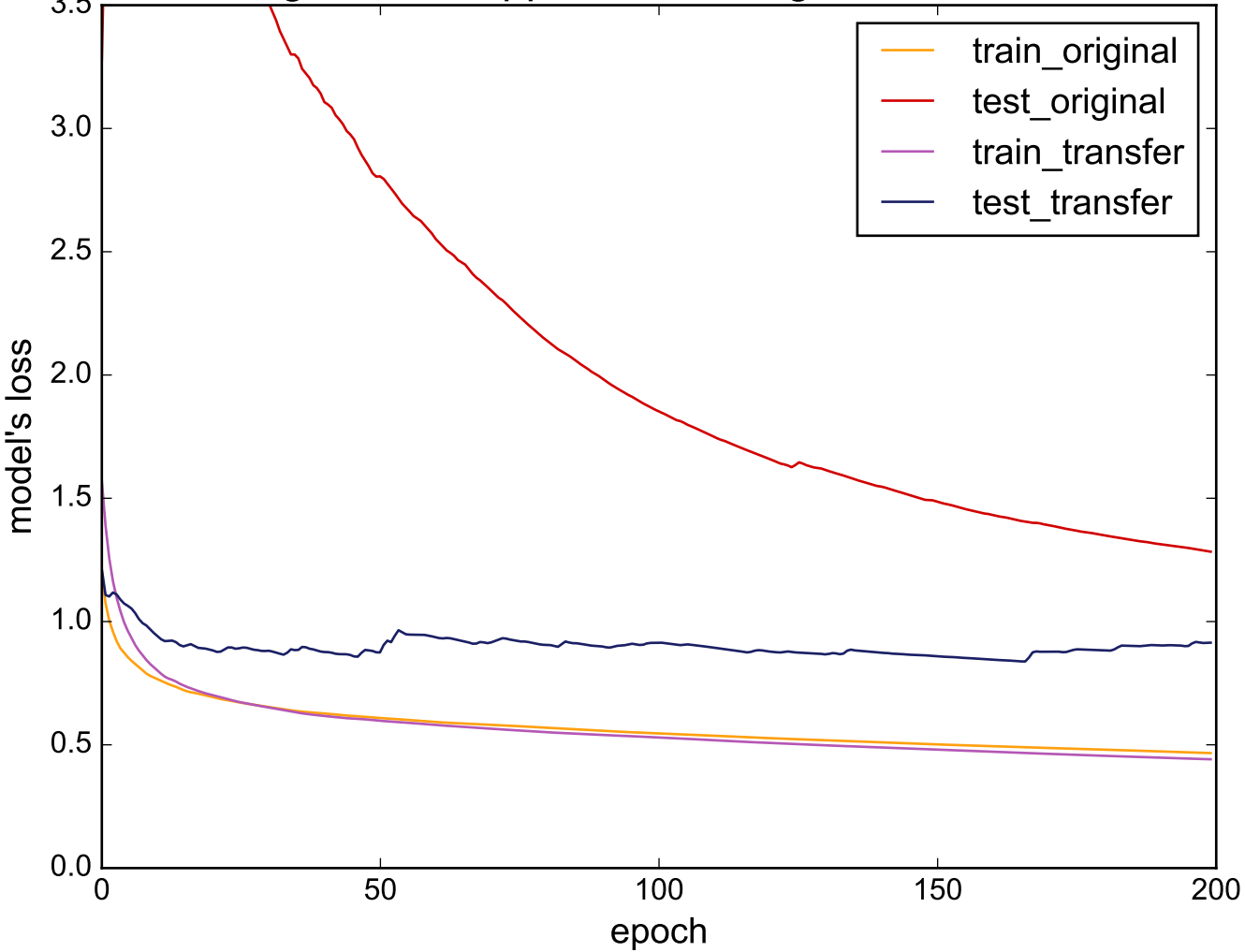
Source: LargeKitchenAppliances - Target: ProximalPhalanxTW
