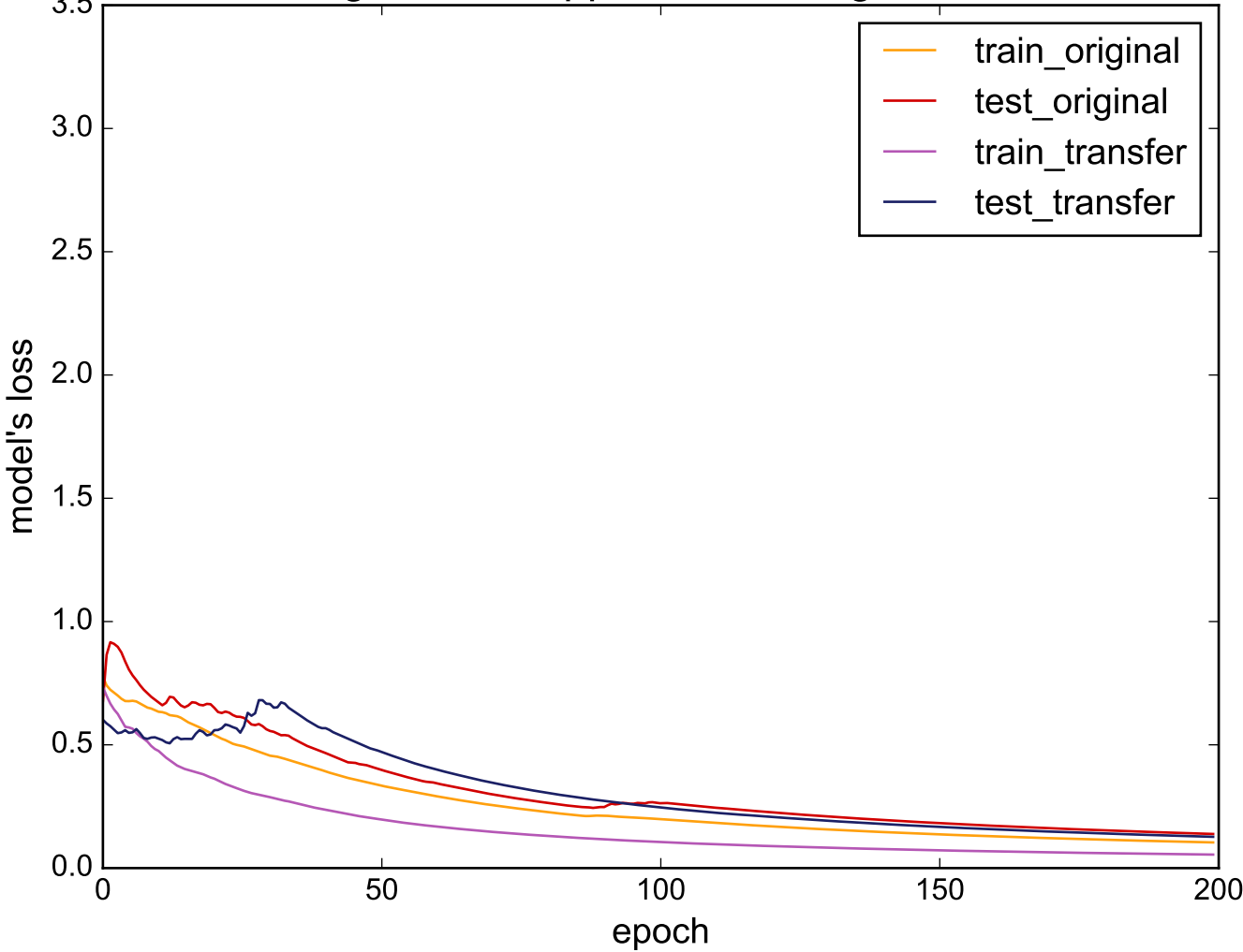
Source: LargeKitchenAppliances - Target: TwoLeadECG
