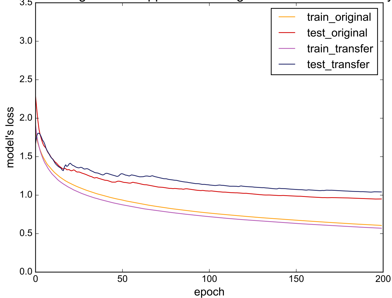
Source: LargeKitchenAppliances - Target: uWaveGestureLibrary_X
