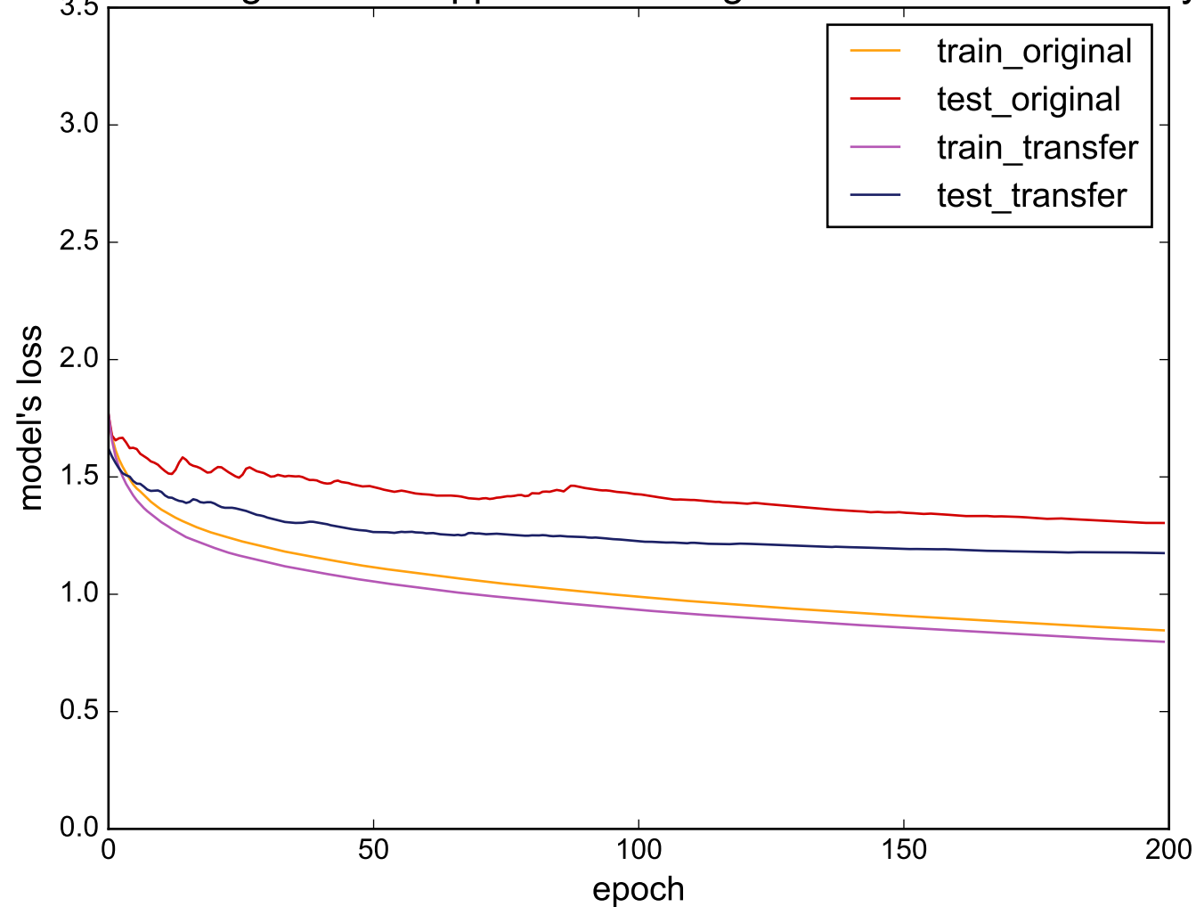
Source: LargeKitchenAppliances - Target: uWaveGestureLibrary_Y
