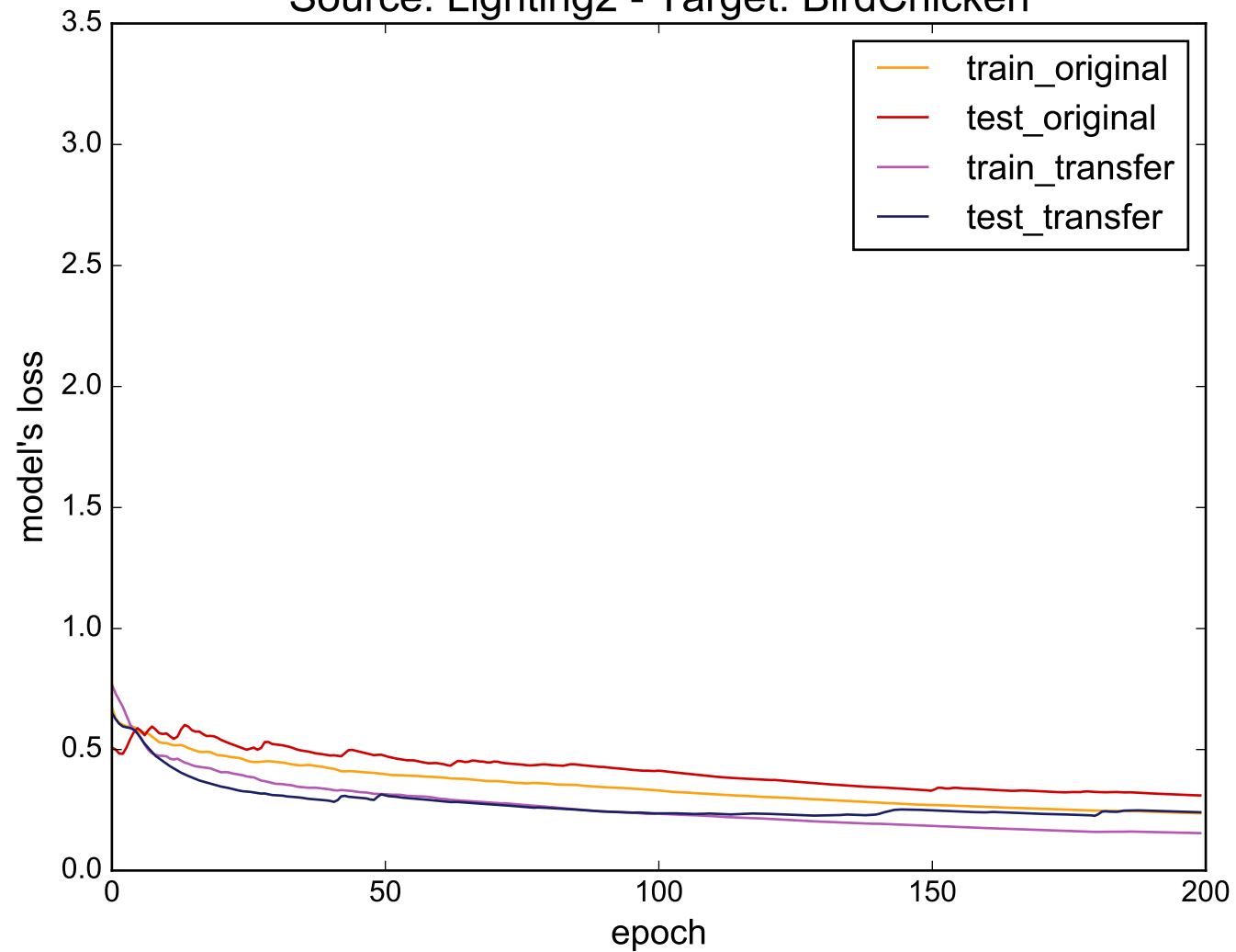
Source: Lighting2 - Target: BirdChicken
