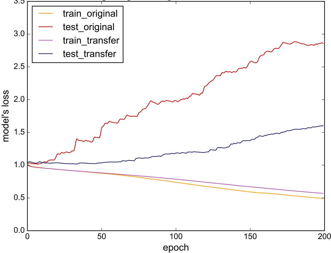
Source: Lighting2 - Target: ChlorineConcentration
