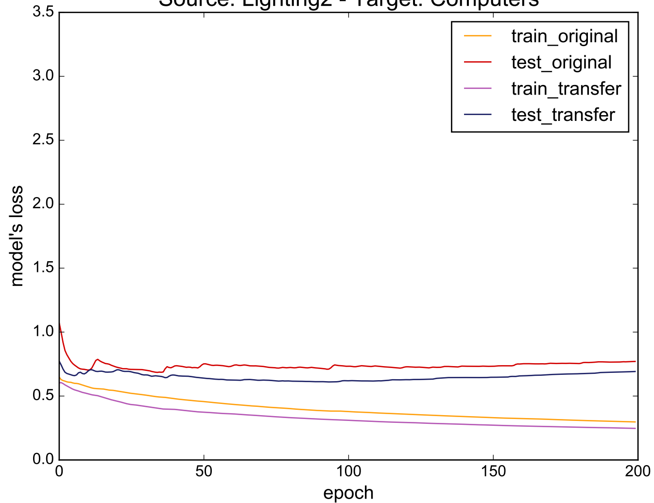
Source: Lighting2 - Target: Computers
